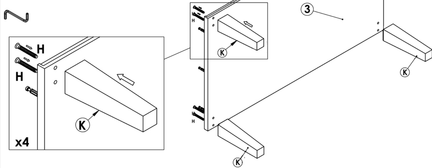
FRONT VIEW
